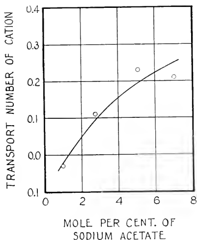
FIG. 2. Apparent transport number of cation in sodium acetate solutions.
